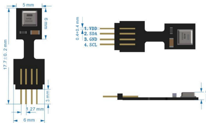
Figure 12. AHT25 sensor encapsulation (unit: mm unmarked tolerance: \pm 0.1mm )
