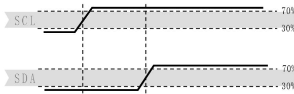
Figure 11. Stop transmission state (P)
